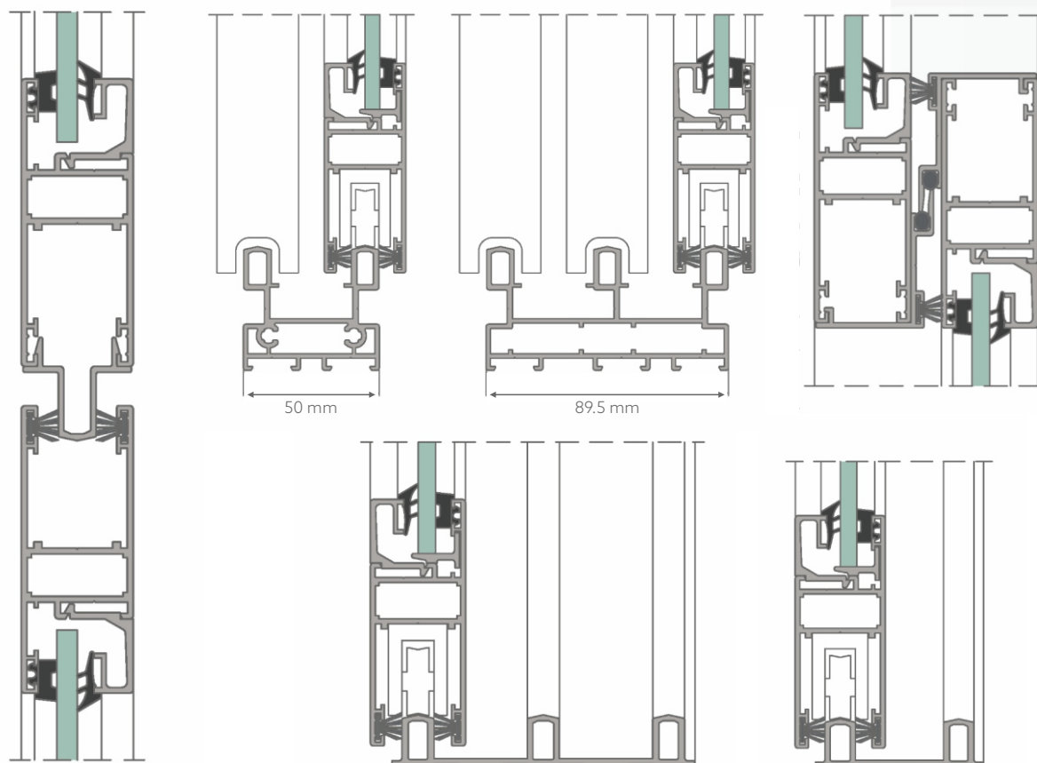
SLIDING LEAF CROSS-SECTION
